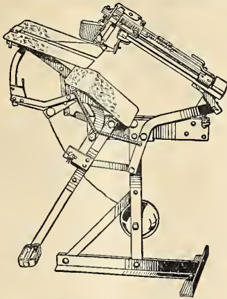
The FELINS Tying Machine
